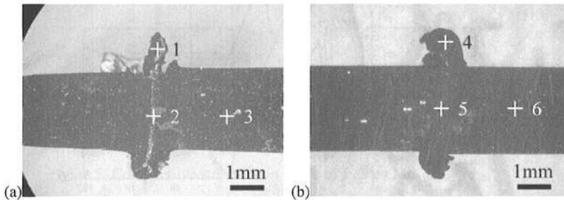
Figure 2. Microstructures of cross section of Mg_{65}Cu_{25}Gd_{10} joints welded at (a) 0.05 MPa and (b) 0.5 MPa. Note that the slight contrasts beside the protrusions were caused by stain adhering to specimens during the desiccation process after polishing.
