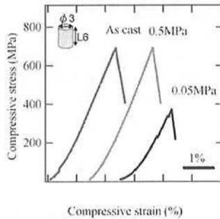
Figure 5. Compressive stress-strain curve of welded Mg_{65}Cu_{25}Gd_{10} .
