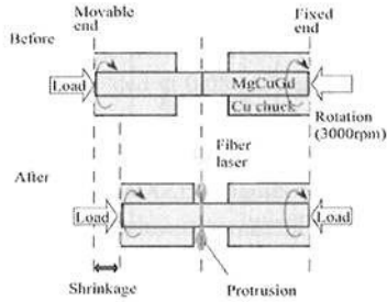
Figure 1. Illustration of laser butt welding of Mg_{65}Cu_{25}Gd_{10} metallic glass.
