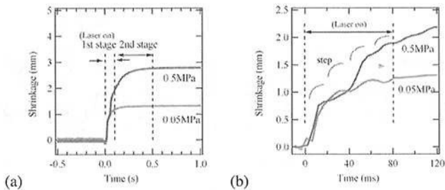
Figure 4. (a) Shrinkage of specimen during laser butt welding. (b) Expanded view from 0 to 120 ms.
