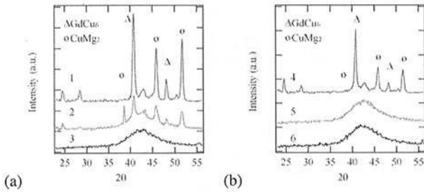
Figure 3. Micro-focused XRD patterns at (a) positions 1, 2, and 3 in Figure 2 and (b) positions 4, 5, and 6 in Figure 2.
