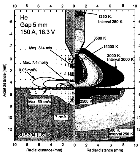
Fig. 4 Calculated results for GTA welding for 150 A (arc gap: 5 mm).
