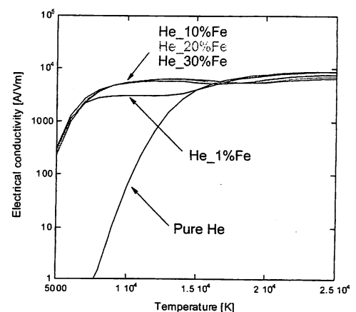
Fig. 2 Dependence of electrical conductivities of helium gas on temperature for each mixing ratio.
