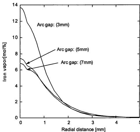
Fig. 6 Radial distributions of iron vapor concentration on the anode.
