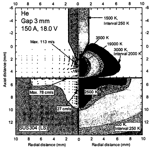
Fig. 7 Calculated results for GTA welding neglecting the effect of iron vapor (arc gap: 3 mm).
