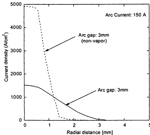
Fig. 8 Comparison of calculated current densities at the anode surface.
