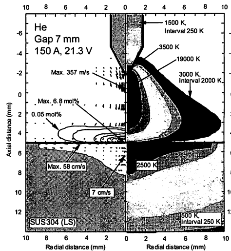
Fig. 5 Calculated results for GTA welding for 150A (arc gap: 3 mm).
