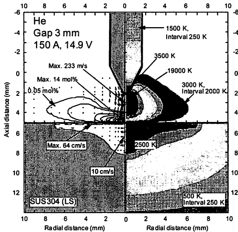
Fig. 3 Calculated results for GTA welding for 150 A (arc gap: 3 mm).
