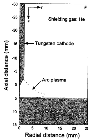
Fig. 1 Schematic illustration of simulation domain (Arc gap: 5 mm).
