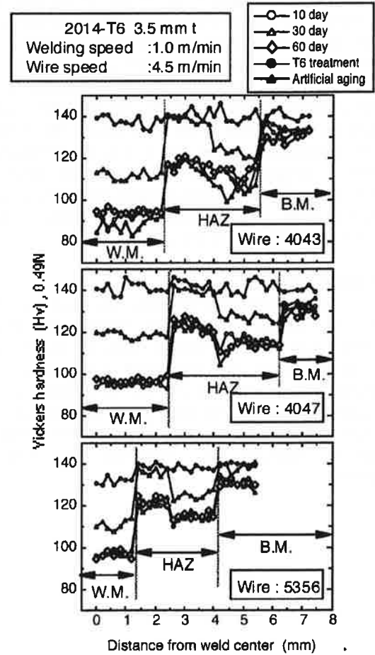
Fig.5 Hardness profiles of laser welded joints.
