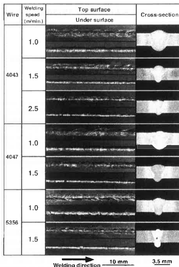
Fig.3 General appearance and macrostructure of cross-sections of laser welded beads.
