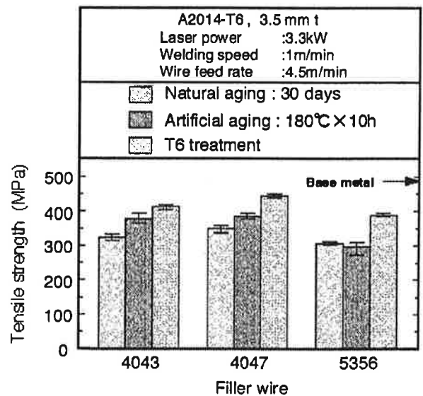
Fig.6 Effect of post-weld heat treatment on tensile strength of laser welded joints with different filler wires.
