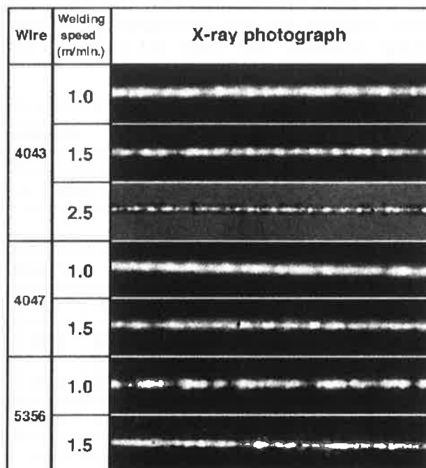
Fig.4 X-ray radiographs of laser welded beads at laser power 3.3kW.
