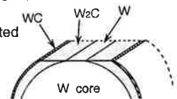
(c) Sketch of specimen (b)
