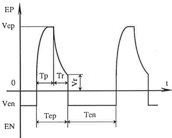
Fig.2 Waveform control for AC-pulsed GMA welder
