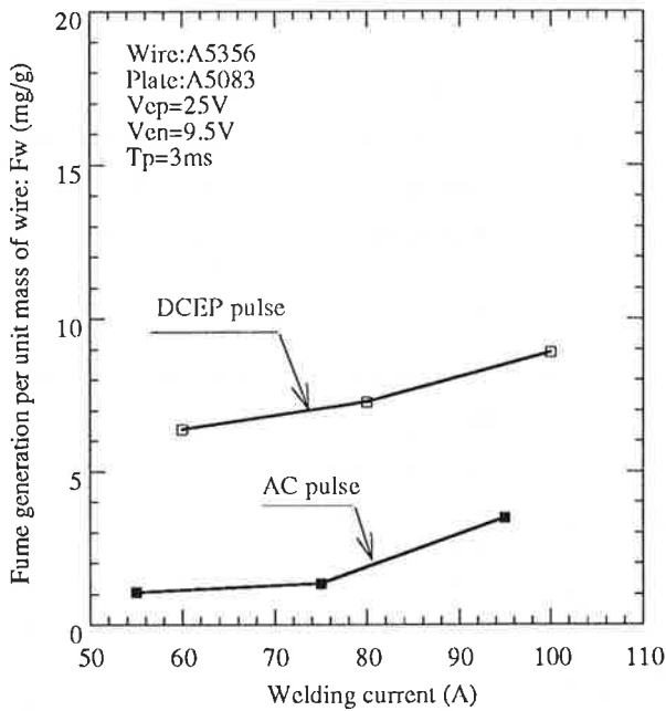
Fig.6 Effect of welding current on fume generation
