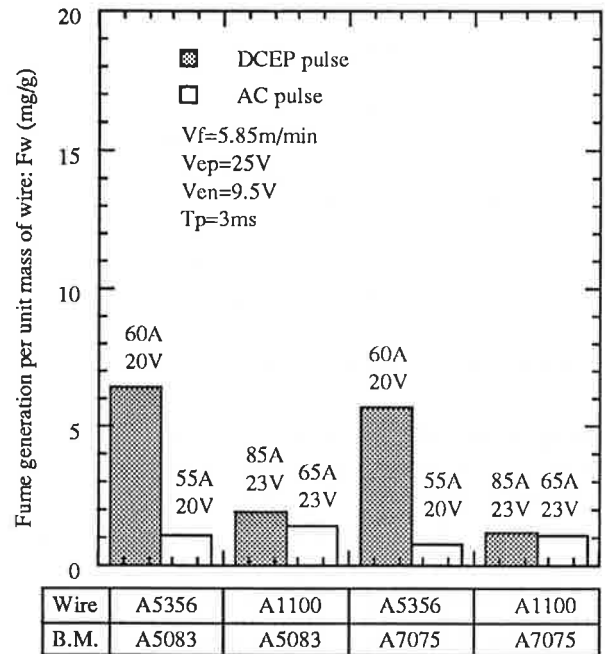
Fig.5 Effect of polarity and welding materials on fume generation
