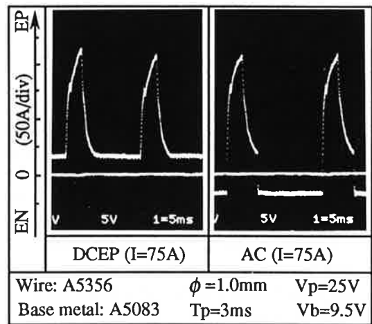
Fig.3 Current waveform of DCEP and AC pulse
