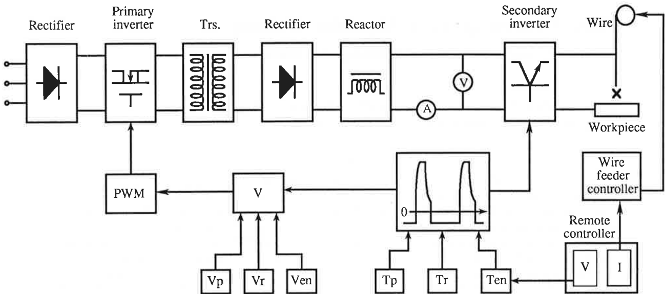
Fig.1 Schematic diagram of the AC-pulsed GMA inverter welder
