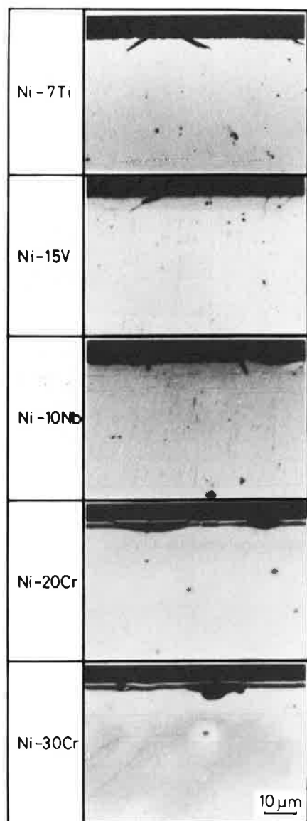
Fig. 6 Microstructure on crosssection of nitrated Ni binary alloys after anodic polarization analysis
