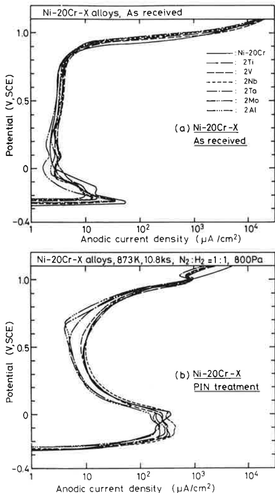
Fig. 4 Anodic polarization curve for Ni-20Cr-X alloys
