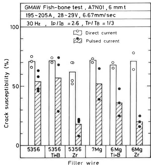
Fig. 5 Effect of current pulsation on crack susceptibility of weld bead for various kinds of filler wires at pulse frequency of 30 Hz for comparison with DC mode.
