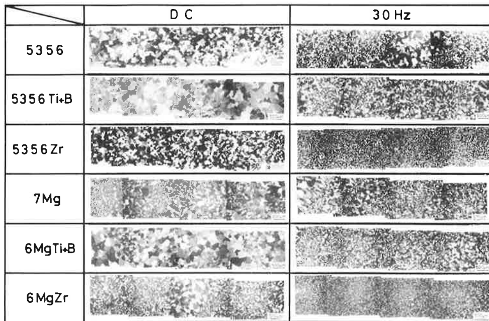
Fig. 6 Grain structural changes caused by current pulsation of 30 Hz for various filler wires.
