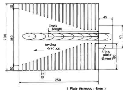
Fig. 2 GMAW Fish-bone cracking test specimen.
