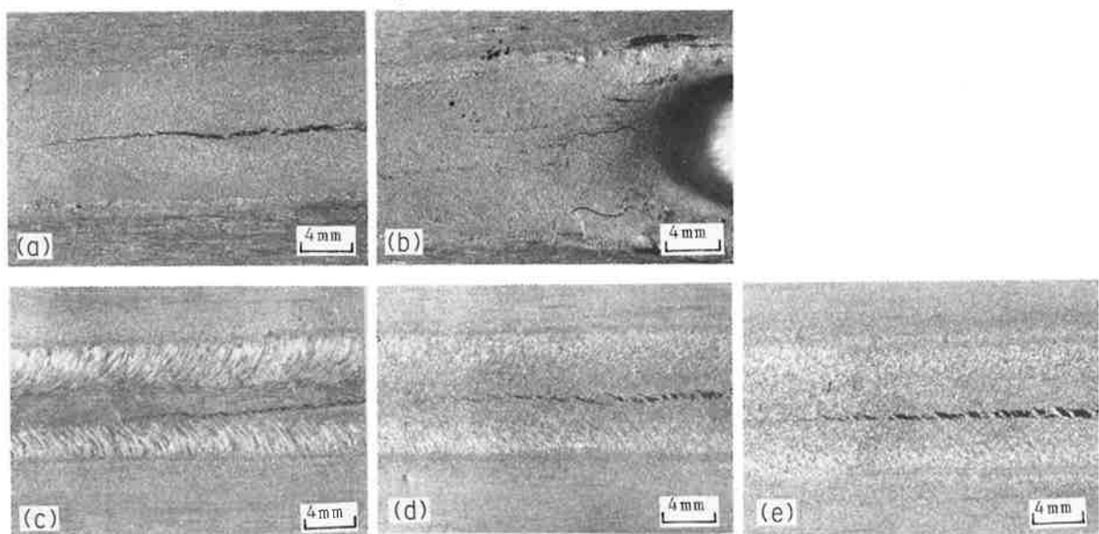
Fig. 11 Macrostructures of the surface of weld bead of Al 2 Zn 3 Mg-0.1Zr base alloy with (a) 0.14%Ti, (b) 0.83%Ti, (c) 0.02% Ti+B, (d) 0.05%Ti+B and (e) 0.07%Ti+B.
