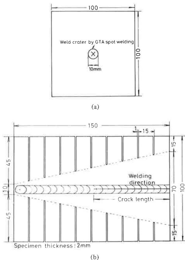
Fig. 1 Configurations of test specimens of (a) GTA weld crater and (b) Houldcroft-type weld bead cracking tests.
