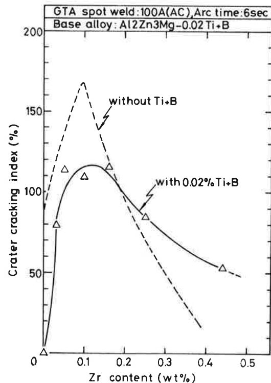
Fig. 4 Effect of Zr addition on crack susceptibility of weld crater of Al 2 Zn 3 Mg base alloy with 0.02%Ti+B in comparison with those without Ti+B.
