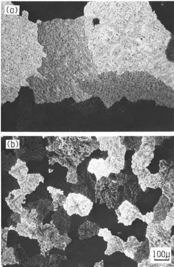
Fig. 8 Typical macrostructures of synthesized-weld-metal alloy with 0.02%Ti+B; (a) without additional Ti, (b) with 0.05%Ti in addition to 0.02%Ti+B
