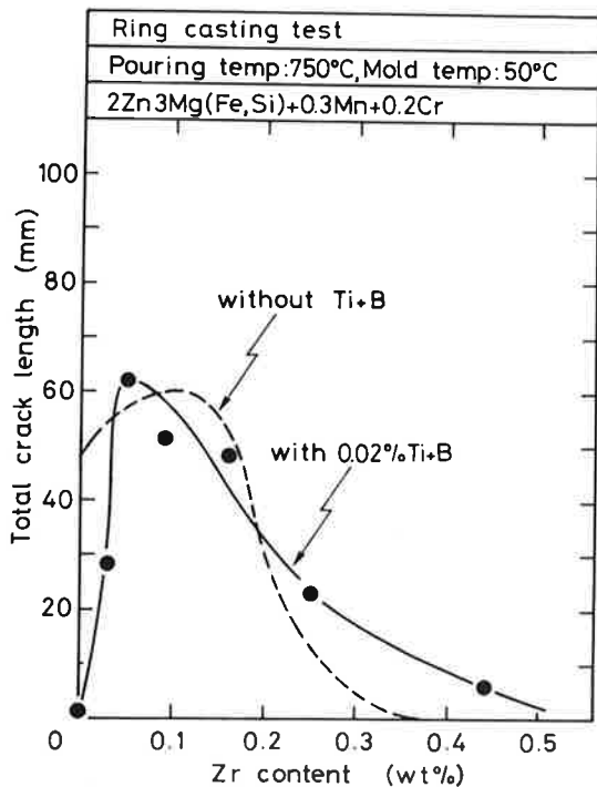
Fig. 5 Effect of Zr addition on total crack length of ring casting of synthesized-weld-metal alloy with 0.02%Ti+B in comparison with those without Ti+B
