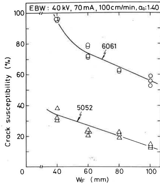
Fig. 3 Effect of width W_F on crack susceptibility of weld bead for 6061 and 5052 6 mm thick alloys with a welding condition of 40kV-70mA-100 cm/min-1.40 a_b .
