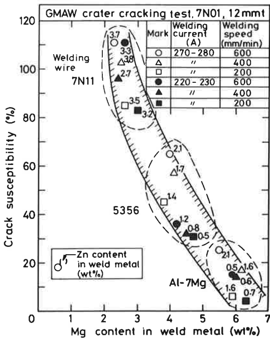
Fig. 23 Effect of Mg content in weld metal on cracking susceptibility evaluated by GMAW crater cracking test.
