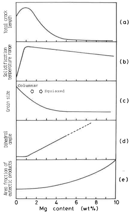
Fig. 20 Schematic diagram showing combined effects of magnesium on cracking susceptibility evaluated by ring-cast cracking test.
