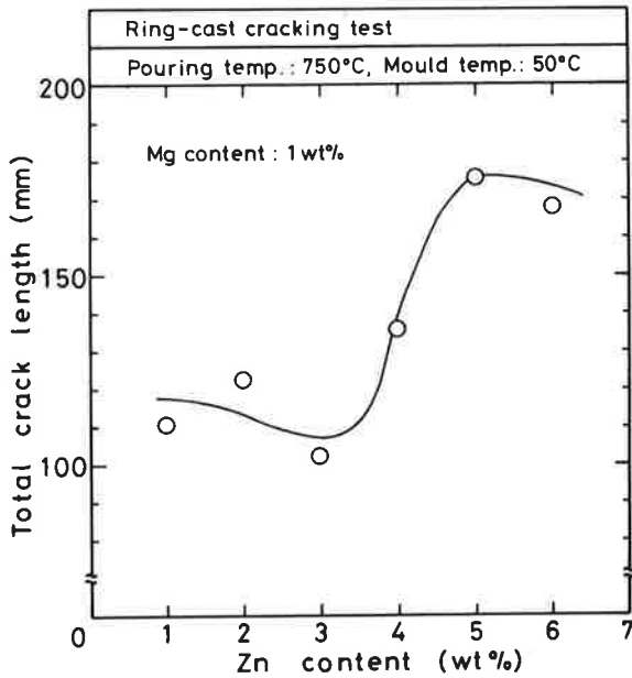
Fig. 7 Effect of Zn content on total-crack length
