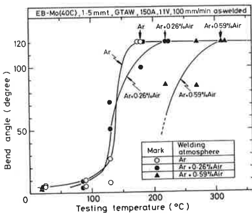
Fig. 5 Influence of air content in welding atmosphere of GTAW on the relations between bend angle and testing temperature for EB-Mo (40C)
