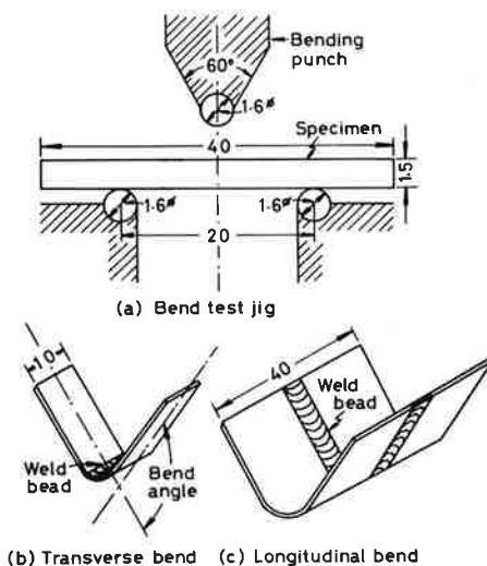
Fig. 1 Nomenclature and dimensions for bend test jig
