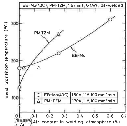
Fig. 7 Effect of air content in welding atmosphere of GTAW on transverse-bend transition temperature for EB-Mo and PM-TZM
