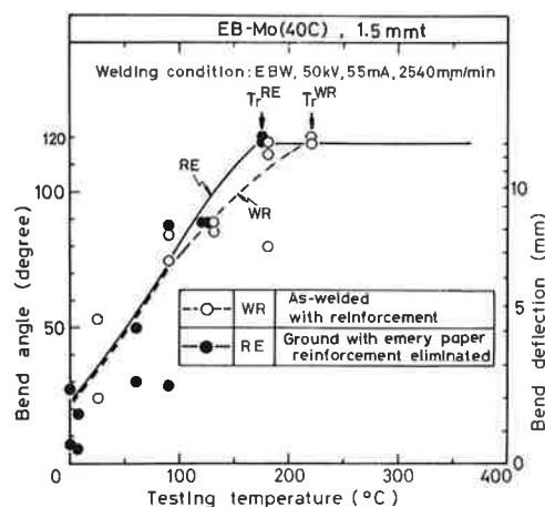
Fig. 10 Influence of surface condition of weld bead on transverse-bend transition temperature for EB welds (material: EB-Mo (40C))
