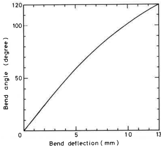
Fig. 2 Relation between bend deflection and bend angle
