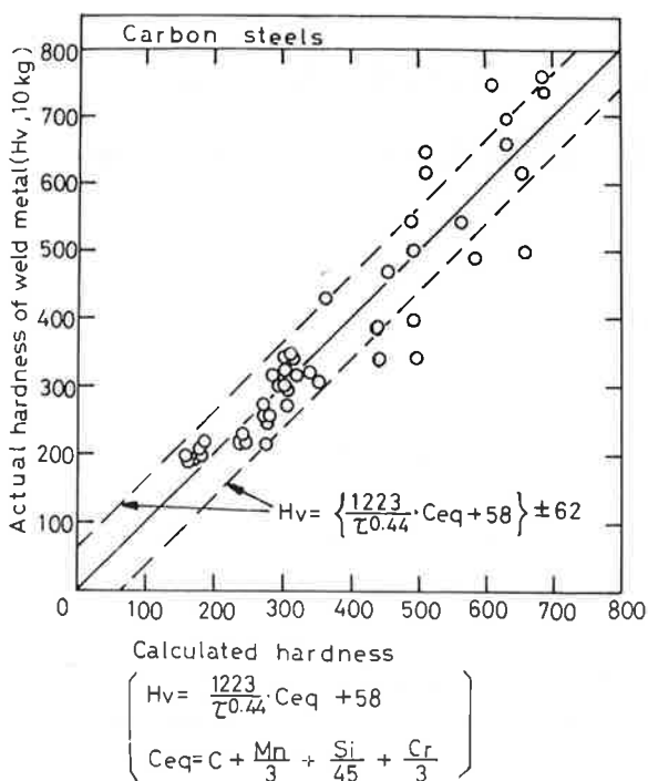
Fig. 2. Comparison of the Actual Hardness with the Calculated Hardness for Electron Beam Weld Metal of the Plain Carbon Steels.
